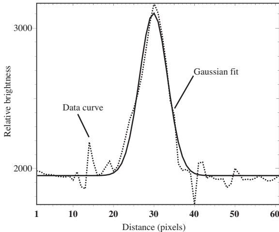
Fig. 5. An example of a Gaussian fit. The dotted curve is the relative brightness across the thin arc and the solid curve shows the Gaussian fit, which gives the FWHM value of the structure. The FWHM value for this fit is 3.5 km and the fit residual 6%.
