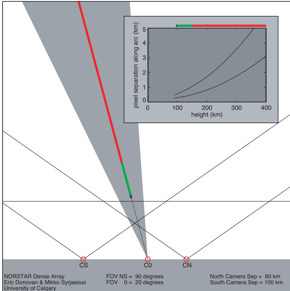
Fig. 1. A possible set-up for altitude profile studies with DAISY. This is a north–south cross-section where south is to the left and north is to the right. The imager in the middle (CO) has a FoV of 20° and looks directly into the aurora along the magnetic field line. The ones on either side, 60 km north of the middle one (CN) and 100 km south of the middle one (CS) have the FoVs of 90° and observe the same structure from the sides. The small panel in the right hand corner of the plot shows the altitude resolution of this set-up: up to the height of about 150 km the pixel separation is less than one kilometre, and up to about 300 km it is still less than 3 km.
