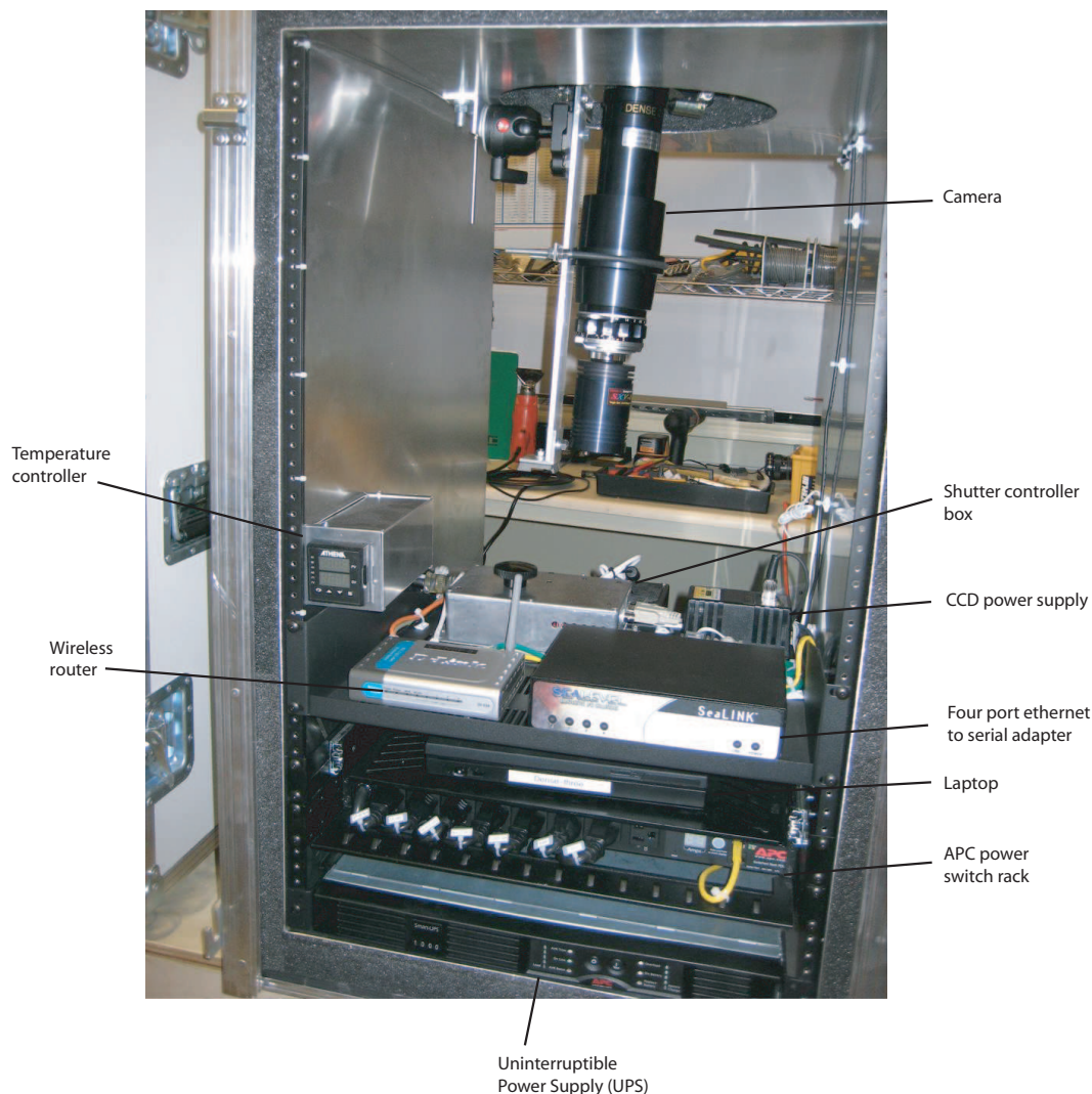
Fig. 3. A photo of the DAISY including the names of the parts inside the camera housing. In addition, there is a small dome and a GPS on the roof of the box.
